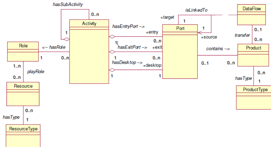
Figure 4 APEL Metamodel [63]
