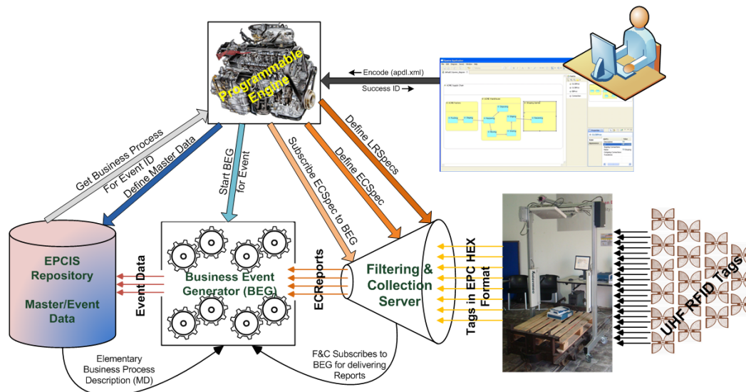
Figure 27 Programmable Engine
