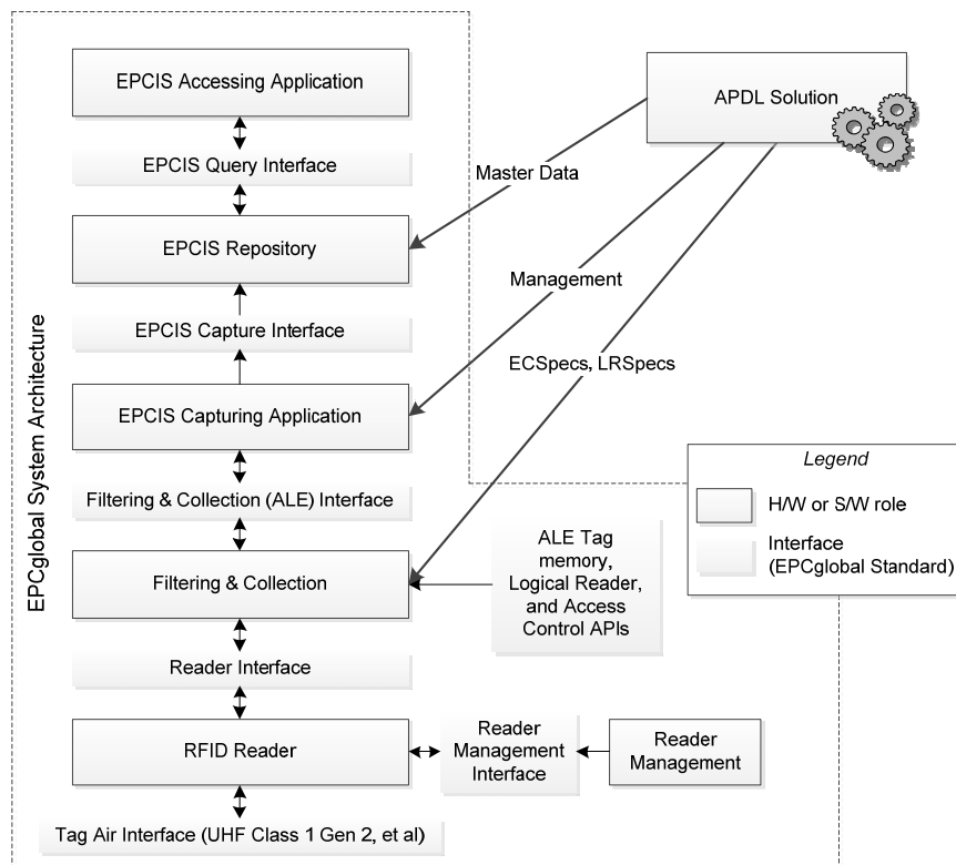
Figure 14 Middle Middleware configuration using APDL [10]
